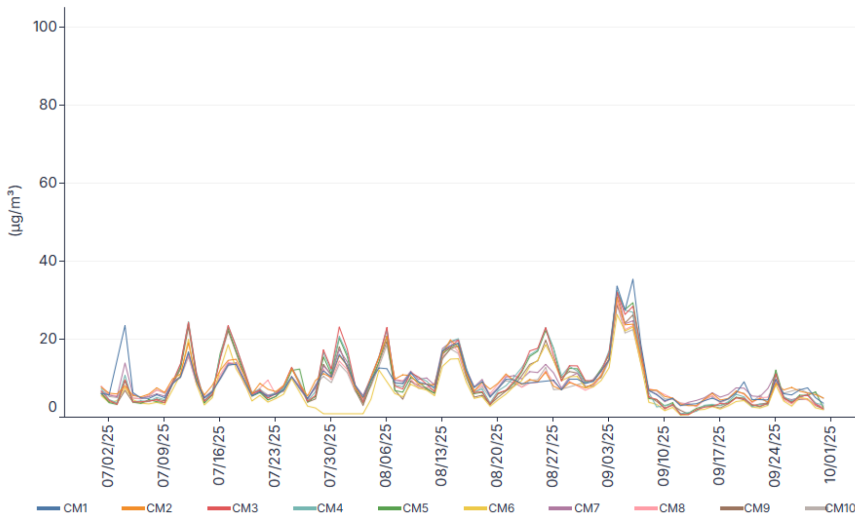
Figure 8 CCND Community Monitoring PM 2.5 24-Hour Block Average Data
