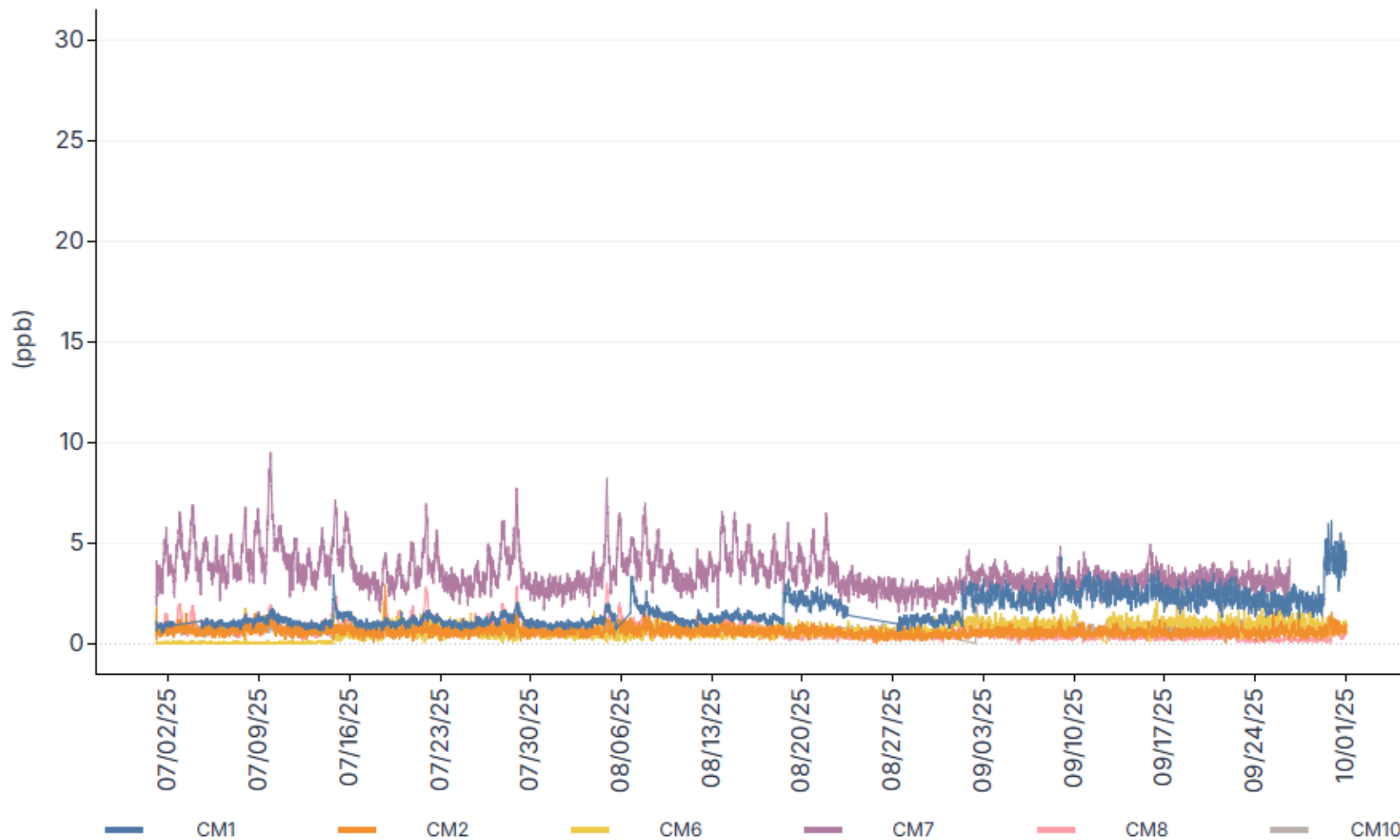
Figure 12 CCND Community Monitoring Ethylbenzene 1-Hour Rolling Average Data 8
